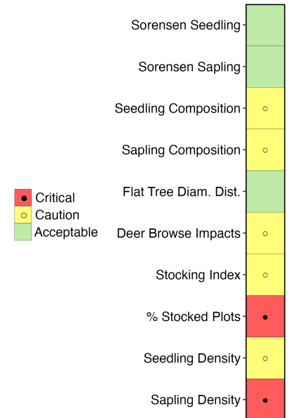
Figure 2. Regeneration status for each of the 10 metrics in Fredericksburg and Spotsylvania National Military Park.
