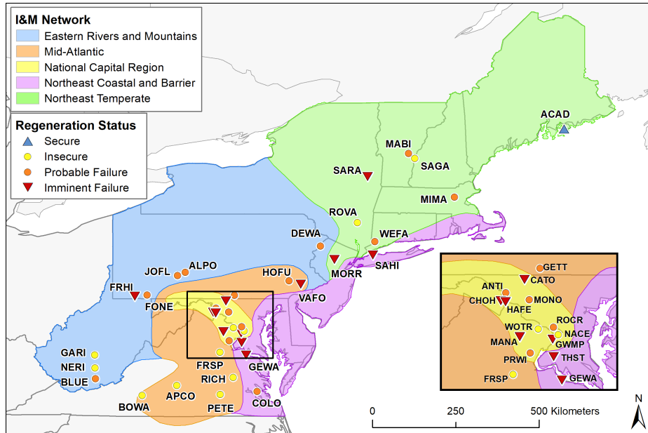
Figure 1. Map of parks included in regional regeneration project and forest regeneration status. Gettysburg National Military Park is located in the Mid-Atlantic (MIDN) Inventory and Monitoring Network.
