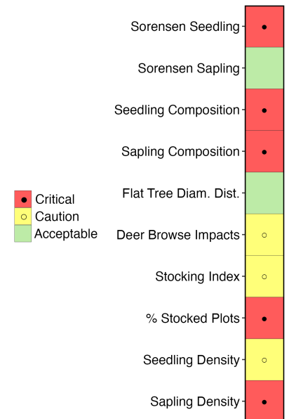
Figure 2. Regeneration status for each of the 10 metrics in Gettysburg National Military Park.
