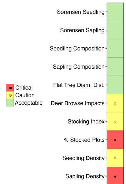
Figure 2. Regeneration status for each of the 10 metrics in Petersburg National Battlefield.
