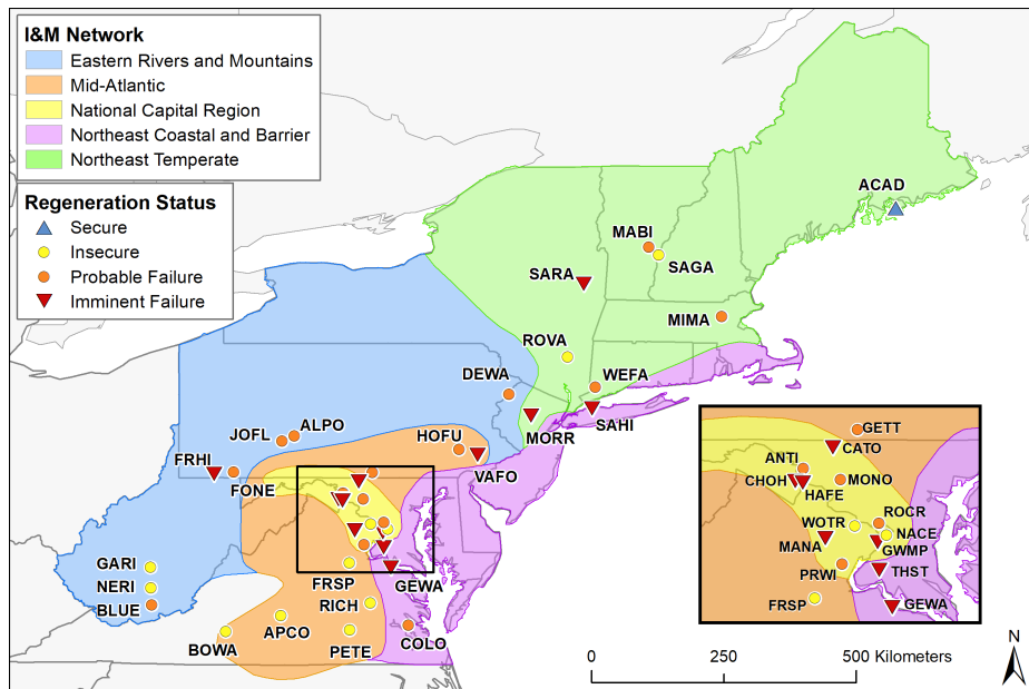
Figure 1. Map of parks included in regional regeneration project and forest regeneration status. Petersburg National Battlefield is located in the Mid-Atlantic (MIDN) Inventory and Monitoring Network.
